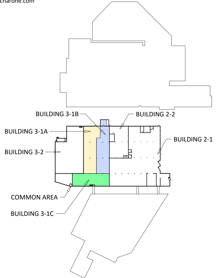
KEY PLAN
