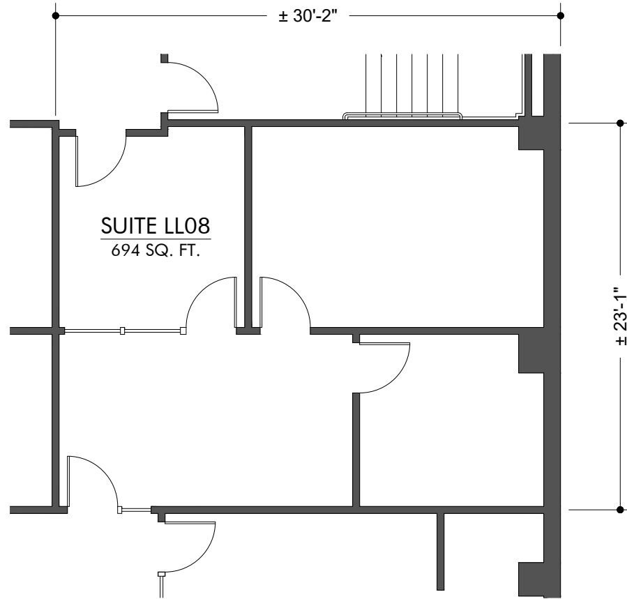
PARTIAL LOWER LEVEL FLOOR PLAN - SUITE LL08 1 W BOYLSTON ST. - WORCESTER, MA
