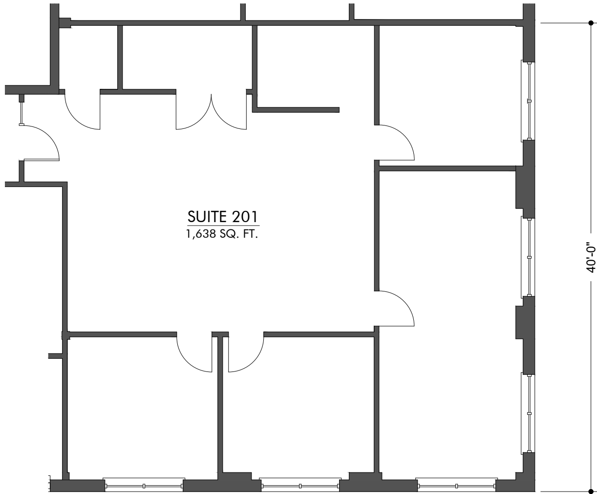
PARTIAL 2nd FLOOR PLAN - SUITE 201 1 W BOYLSTON ST. - WORCESTER, MA
